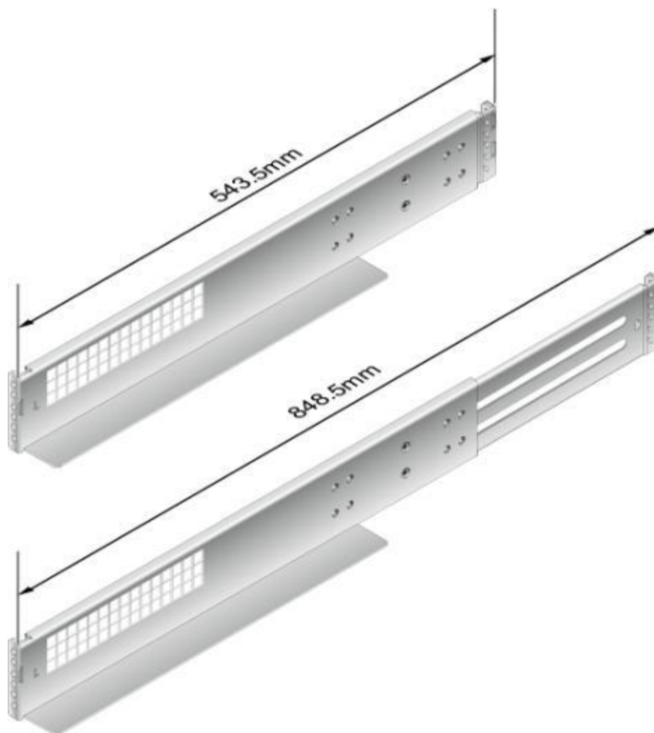
图 6-8 机柜前后方孔条的距离范围
